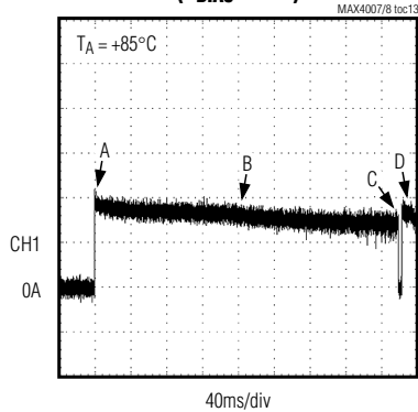
SHORT-CIRCUIT RESPONSE ( V_{BIAS} = 76\text{V} )
